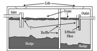
Cross-section of a two-compartment septic tank
